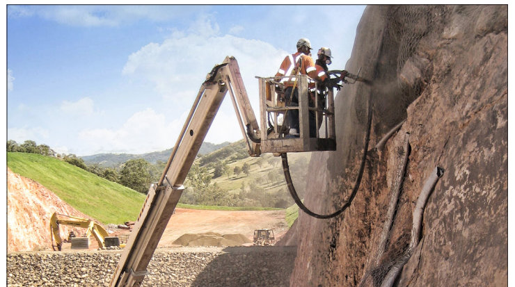
Highwall bolt-mesh and shotcrete application.
